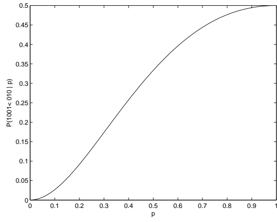
Figure 4: \mathbb{P}(1001 \prec 010|p) .
