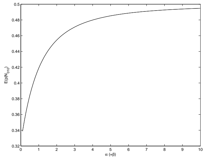
Figure 2: E(p|N_{010} = 10) for different values of \alpha .
