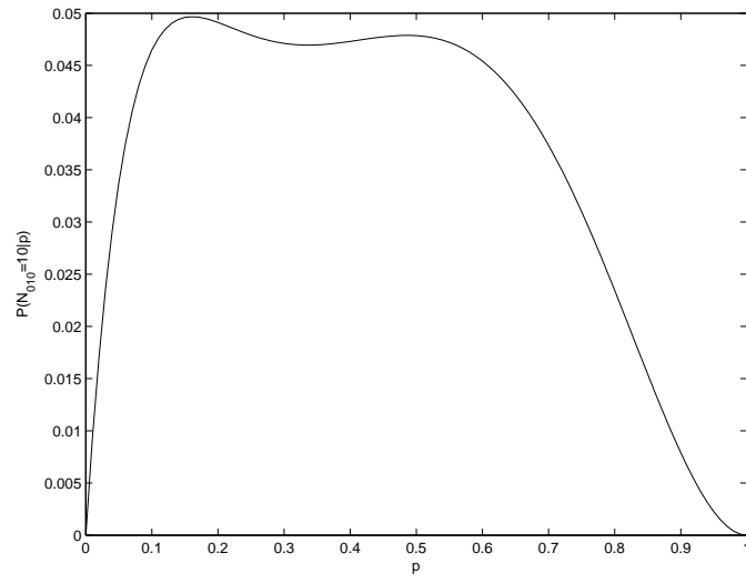
Figure 1: Likelihood P(N_{010} = 10|p)
