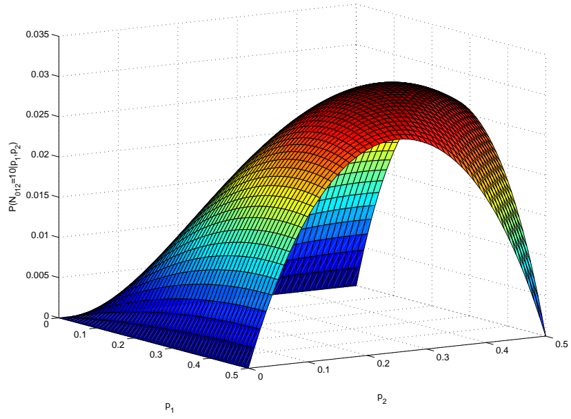
Figure 3: P(N_{012} = 10 | \mathbf{p}) for different values of \mathbf{p} .
